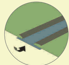
STEP 05 Fold the trimmed edges; Put the width joint tape below the edges
